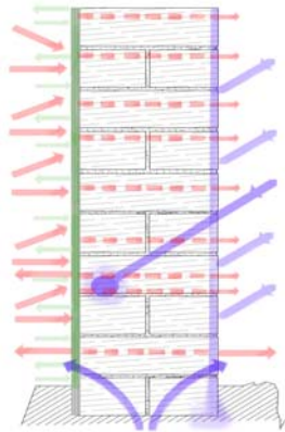
Victorian Solid 9" brick wall with limeplaster and distemper internally
